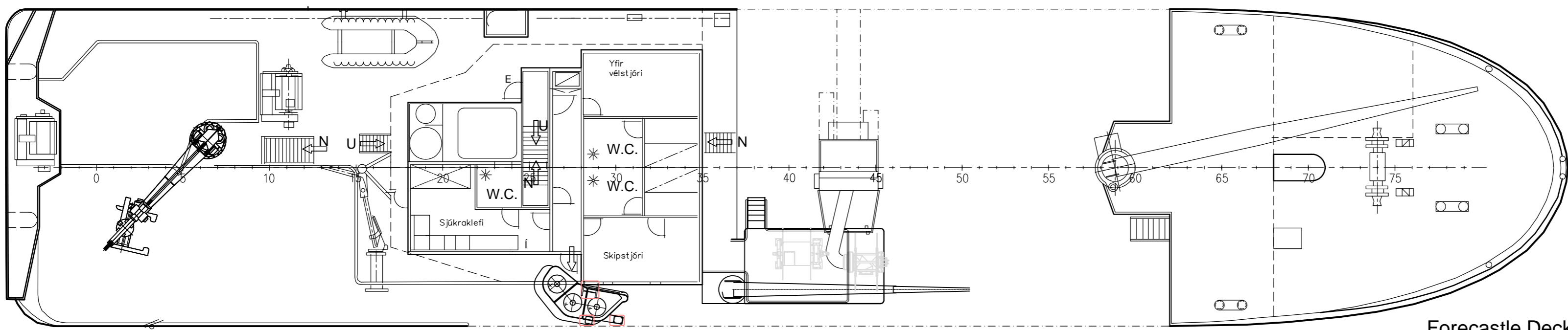
Forecastle Deck
