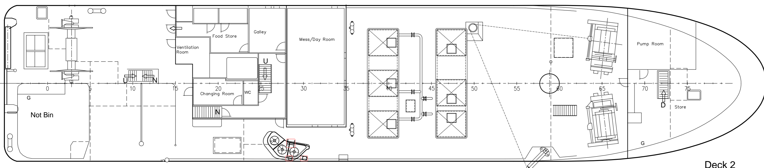
Deck 2
