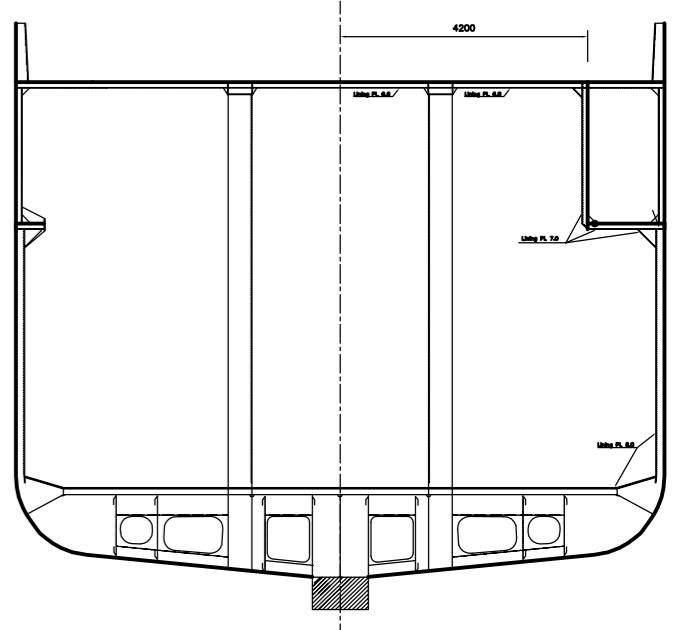
Section frame 45
